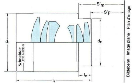
CINE-XENON 2/110-2,3/ 150 mm MC Ø 70,65
