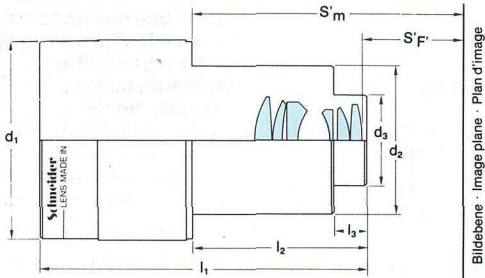
CINE-XENON 2/60- 105 mm MC Ø 70,65
