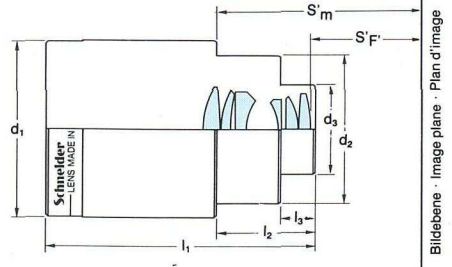
CINE-XENON 2/55- 110 mm MC Ø 62,5
